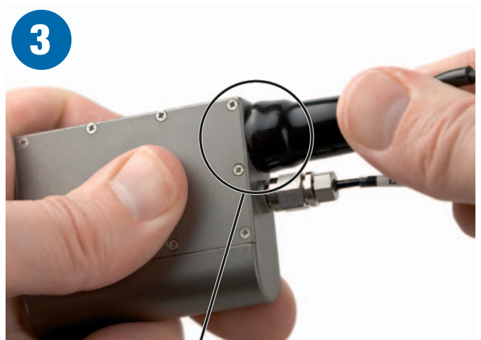
3 Slide the sleeve over the connector. Pinch and squeeze the sleeve near the flange and work it down with a kneading motion over the flange all the way around until it stays in place flush with the housing. Pull on the connector to make sure it is firmly latched.
